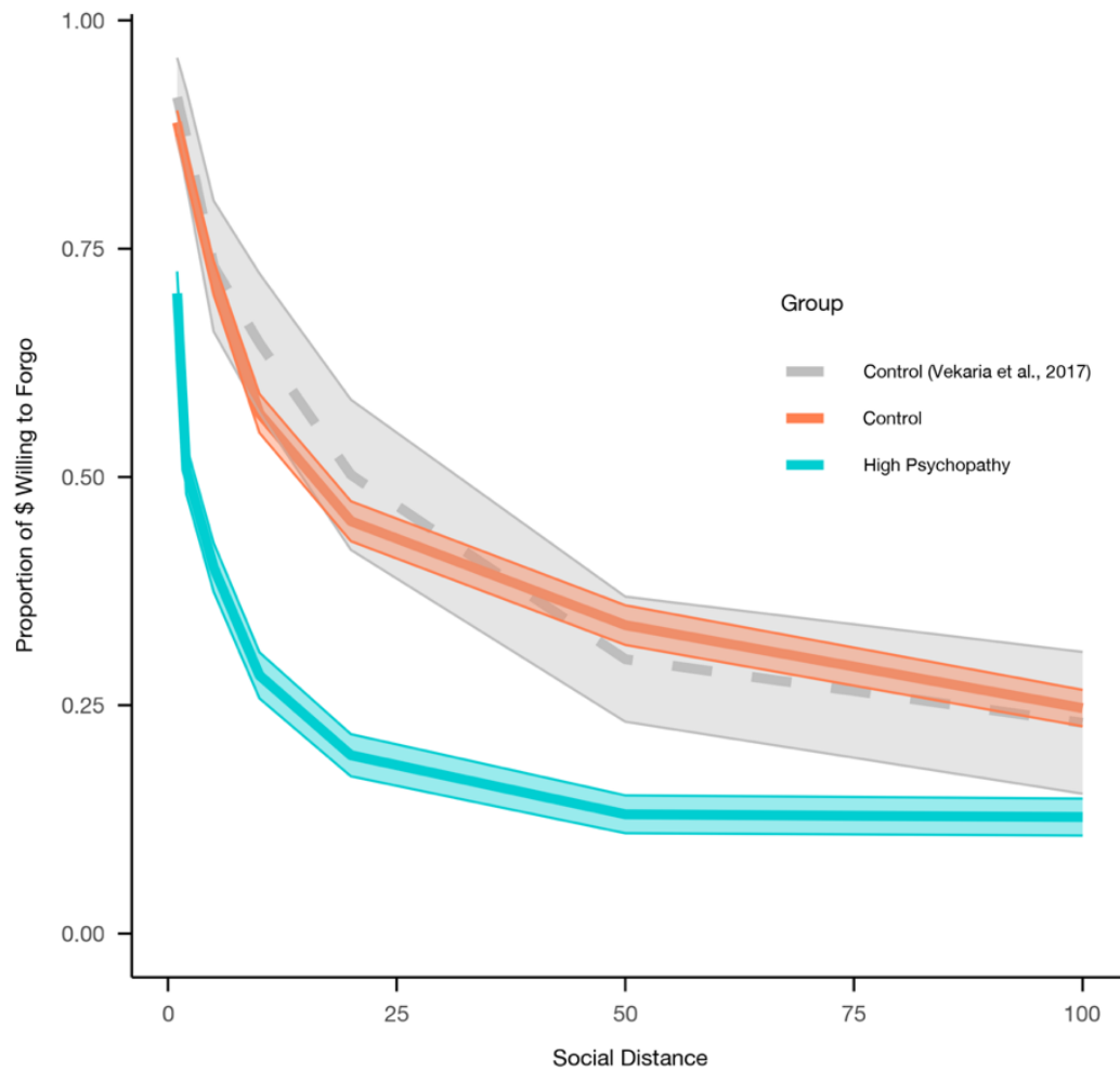
Figure 3 (from Nero et al., 2025) Hyperbolic Social Discounting Curve Across Studies
